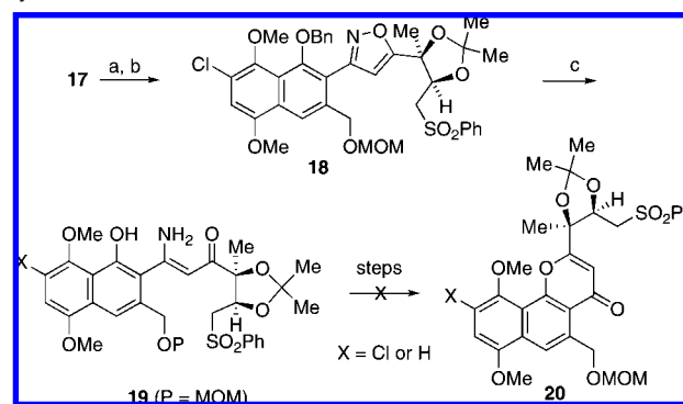
Scheme 4. Synthesis of Enamide 19 and Failed Conversion into Pyrone 20 a
