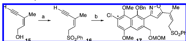
Scheme 3. Synthesis of Isoxazole 17 a
