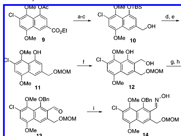
Scheme 2. Synthesis of Oxime 14 a
